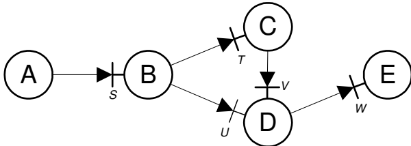
Figure 4. A web of objects collaborating through roles
